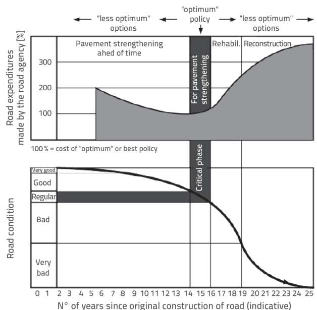
Figure 1. Optimum and less optimum intervention options – road agency costs [25]
