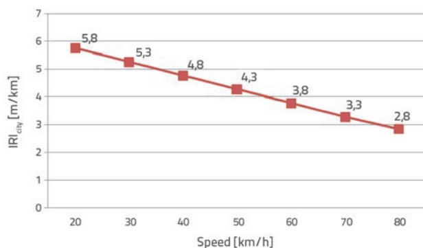
Figure 2. IRI_{city} threshold for different speeds
