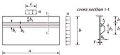
Figure 21. Definition of plate dimensions, boundary conditions and load
